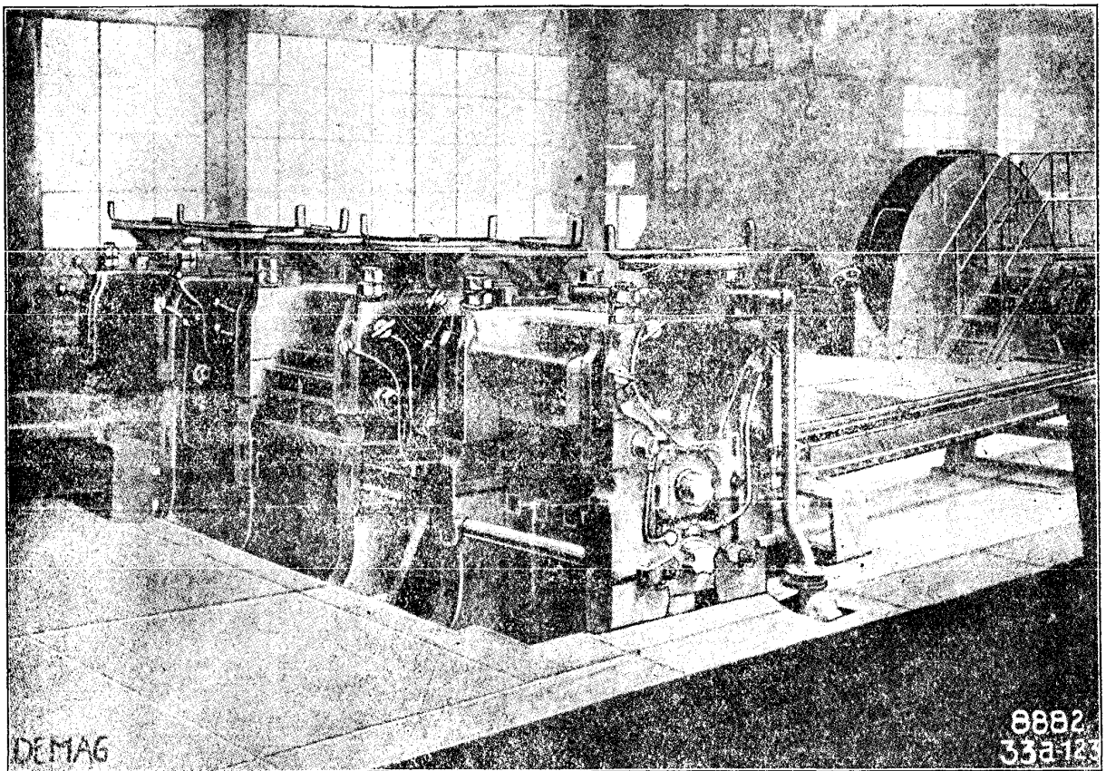
Wire Mill with Roll pin-Roller bearings.
