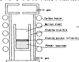
Fig. 1 Experimental apparatus.
