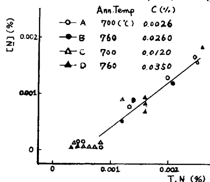
fig. 2 Total N contents vs. N in solution.
