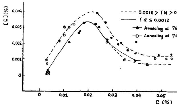
fig. 1 Total C contents vs. C in solution.
