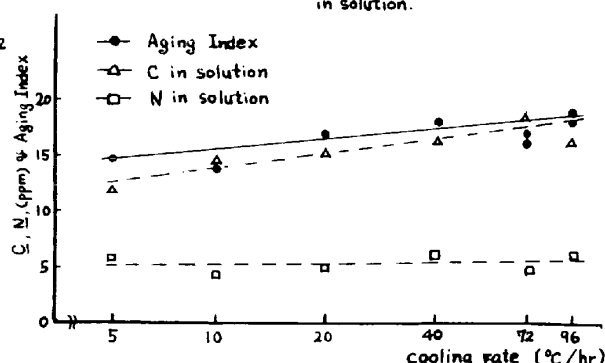
fig. 5 Relation between cooling rate and C, N or Aging Index.
