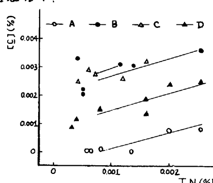
fig. 3 Total N contents vs. C in solution.
