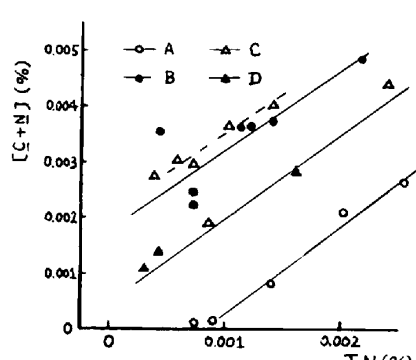
fig. 4 Total N contents vs. C+N in solution.
